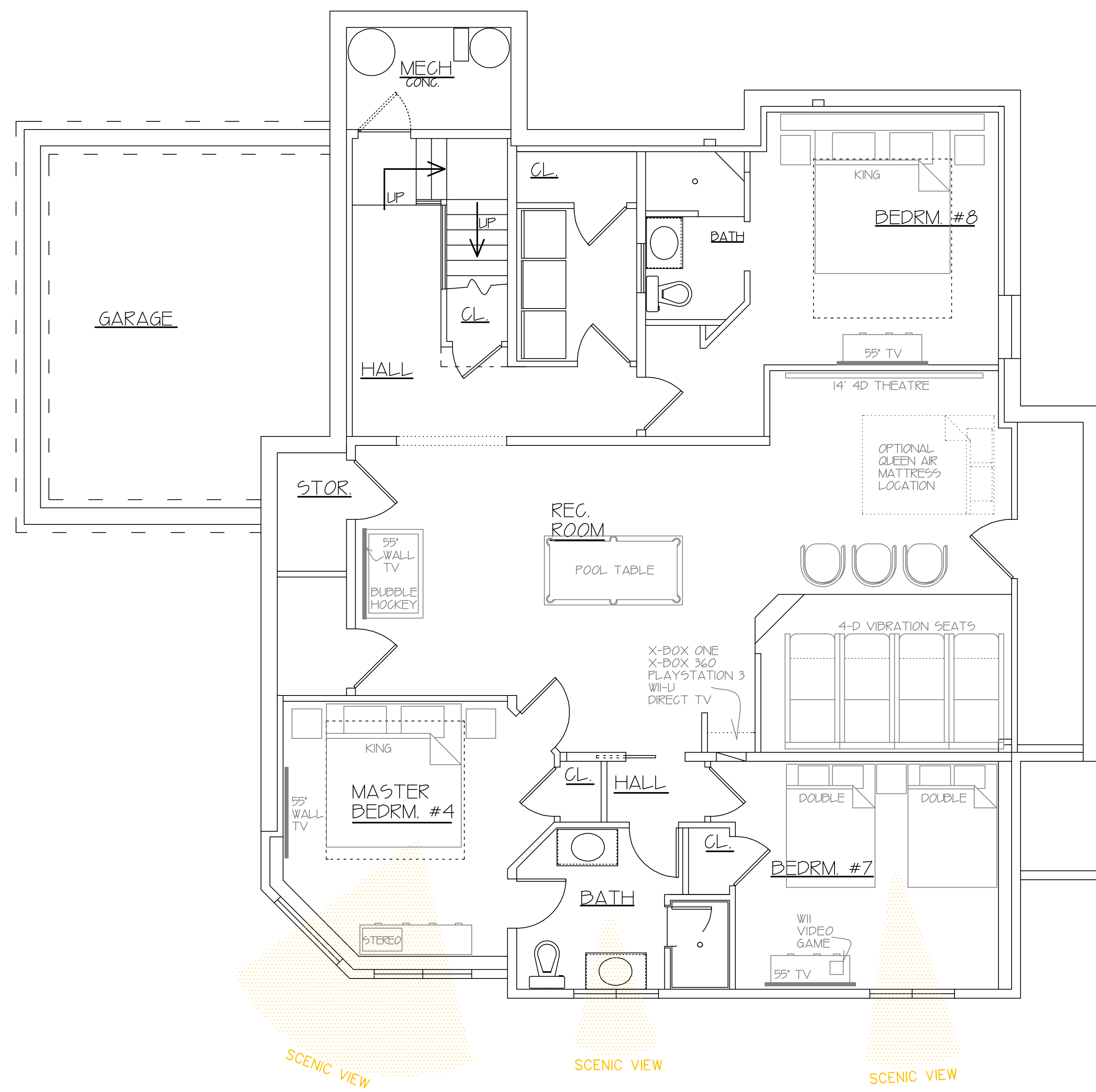
LOWER FLOOR
