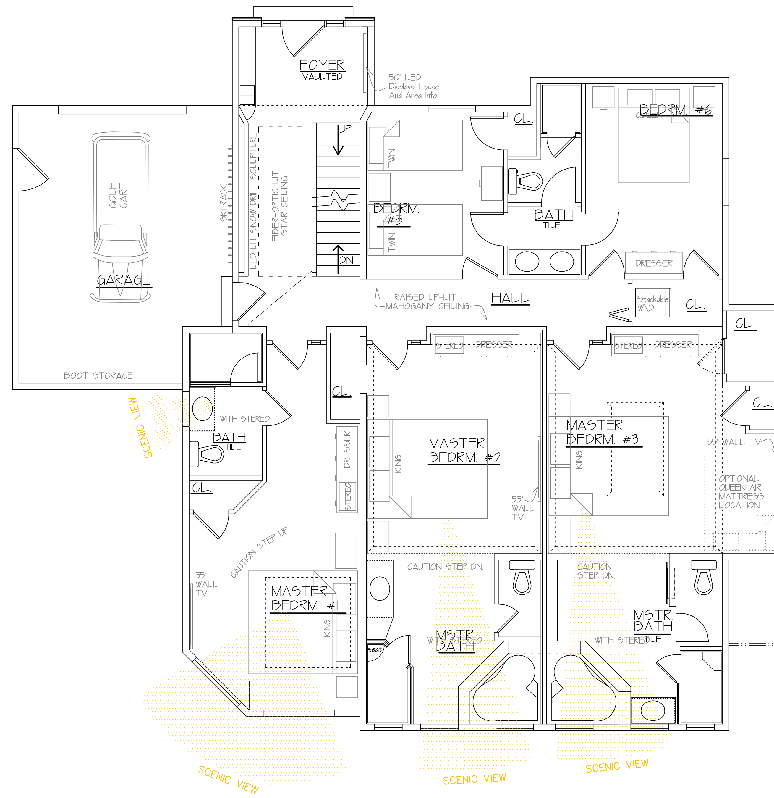
FIRST FLOOR
